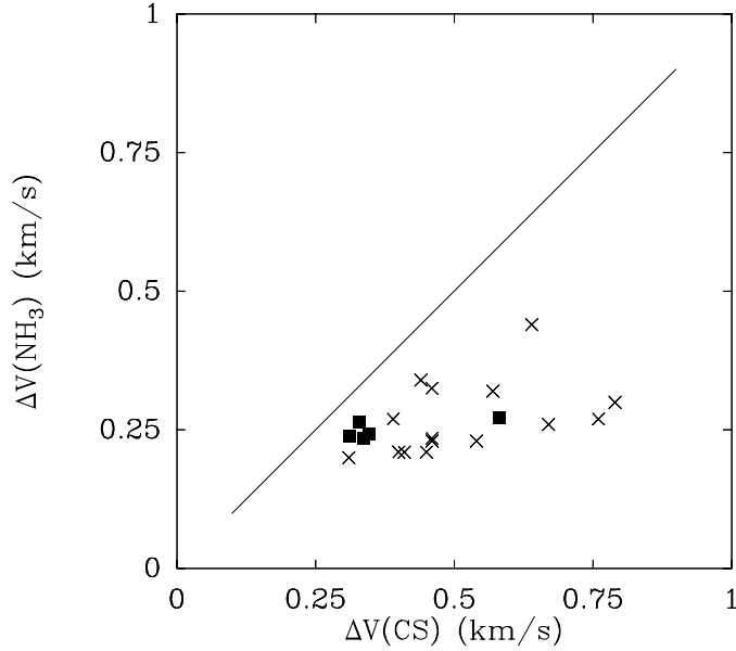
FIG. 9.— Comparison of CS and \text{NH}_3 linewidths from dense cores. Crosses are data from Zhou et al. (1989) (starless cores only), and filled squares are results from our Monte Carlo models. Both real data and models lie below the line of equal CS and \text{NH}_3 linewidth, implying that CS lines are systematically broader than \text{NH}_3 lines. Although this linewidth discrepancy has been traditionally interpreted as resulting from the systematic increase of gas turbulence with core radius, none of our models has this property. Optical depth broadening and self absorption are the two causes of the broader CS lines in the Monte Carlo models (see text).
